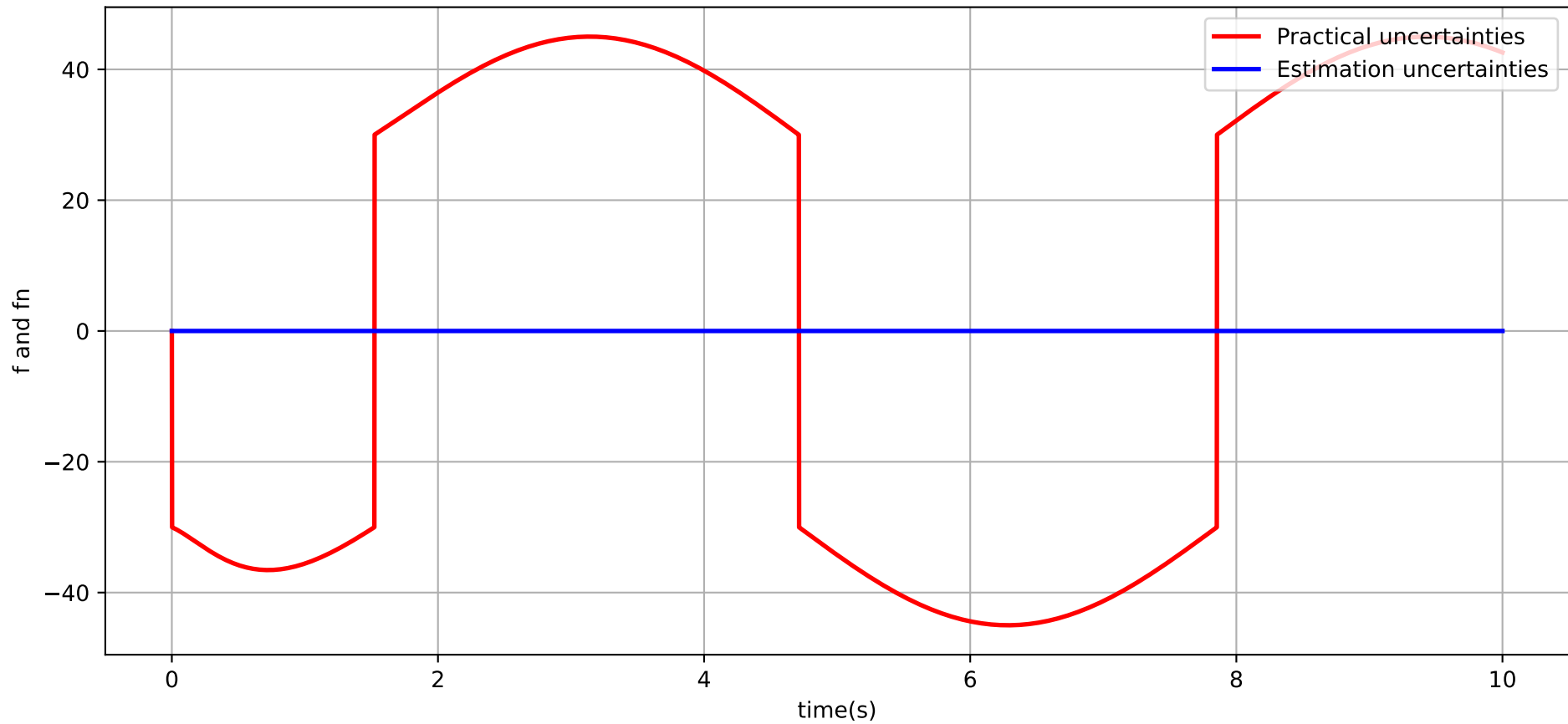
Disturbance Estimation Performance ( S=2 , S1=1 , m=19 )
